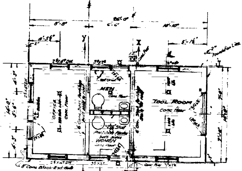
PLAN Scale 1/4" = 1'
