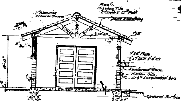
SECTION A-A Scale 1/4" = 1'
